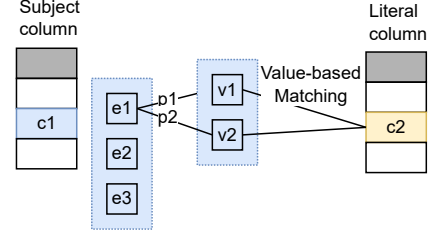
Fig. 6. Illustration of candidate property generation between the subject column and a literal column
