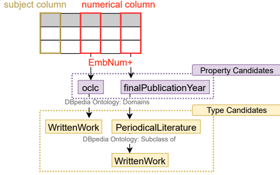
Fig. 4. Property lookup with EmbNum+
