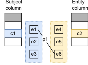
Fig. 5. Illustration of candidate property generation between the subject column and an entity column.
