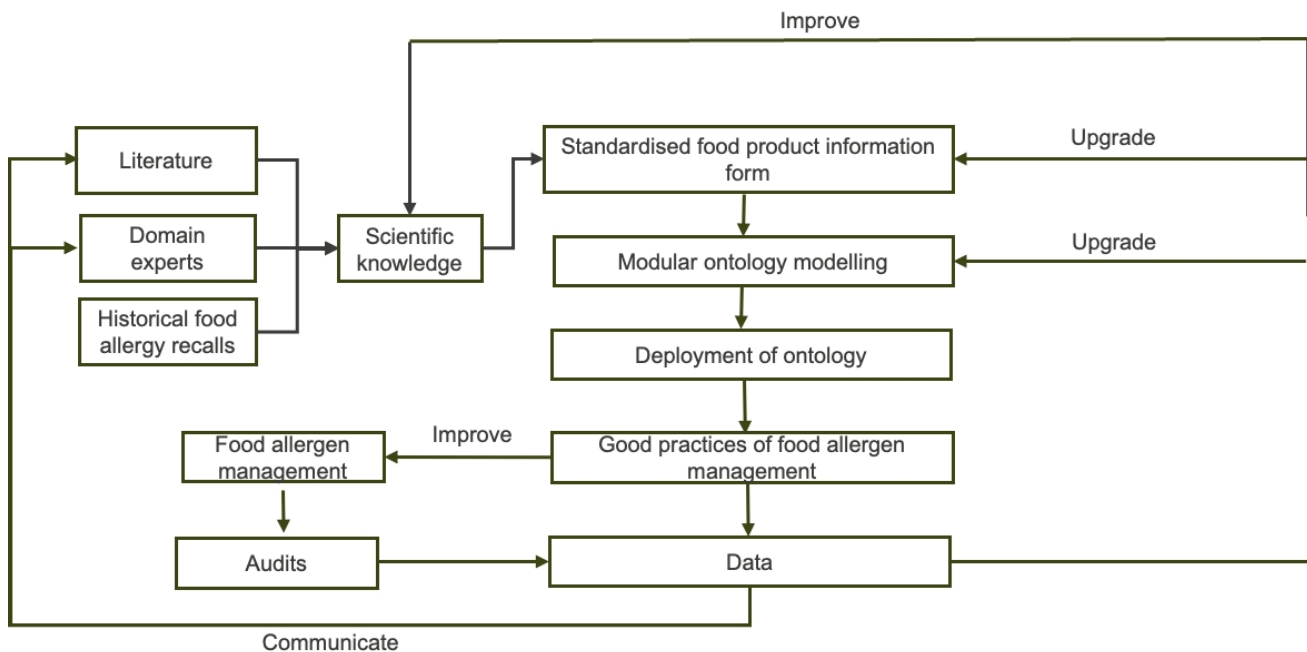
Figure 1. Integrating scientific knowledge for developing and maintaining FATO
