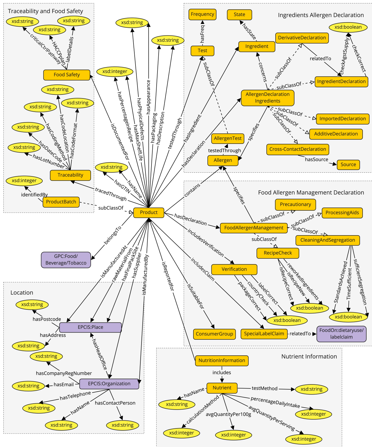
Figure 2. Schema diagram for FATO, with classes from external sources shown in purple.
