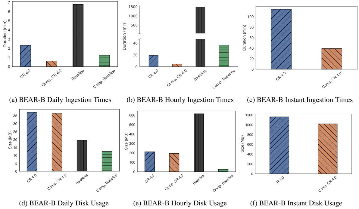
Fig. 10. Ingestion times (top row) and disk usage (bottom row) for OSTRICH and a multi-snapshot storage strategy applied on the different BEAR-B flavours with the original version metadata representation and our new compressed representation.
