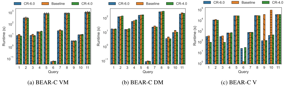
Fig. 13. BEAR-C average query execution time in seconds for VM, DM, and V queries. (log scale)
