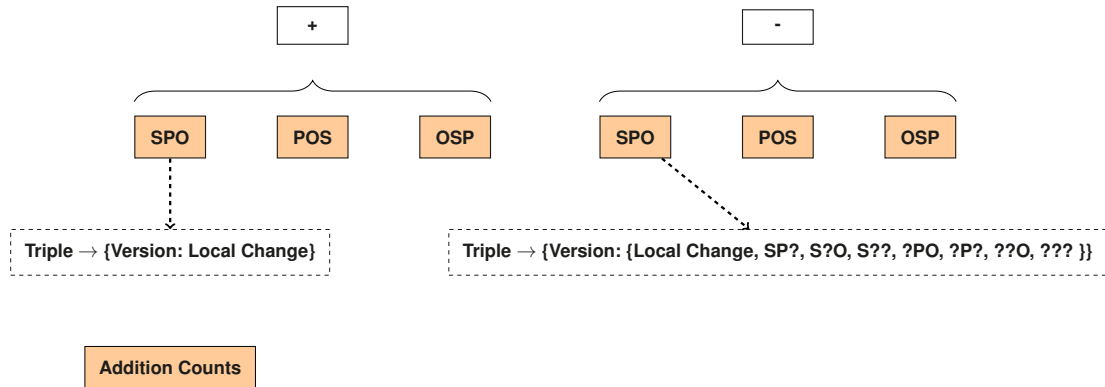
Fig. 2. OSTRICH Delta Chain Storage Overview
