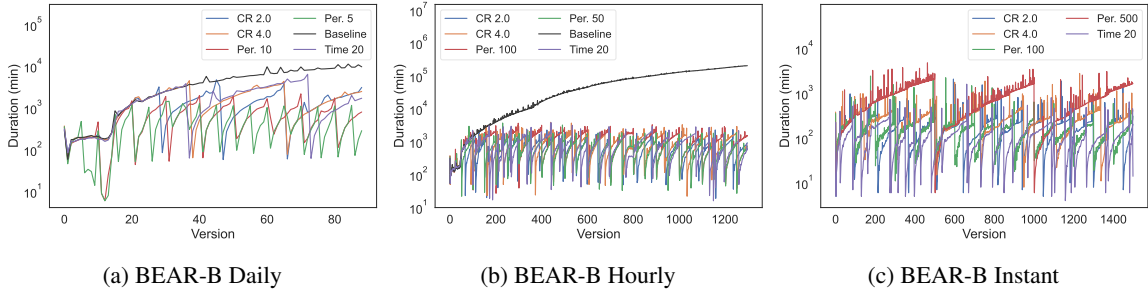
Fig. 7. Detailed ingestion times (log scale) per revision. We include the first 1500 revisions for BEAR-B instant since the runtime pattern is recurrent along the entire history.
