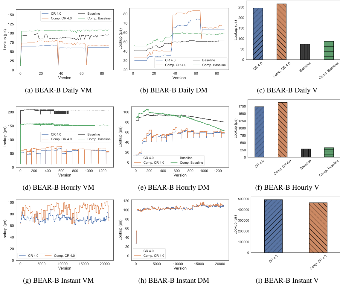
Fig. 12. Query results for the BEAR benchmark with the original version metadata encoding and the new compressed encoding.
