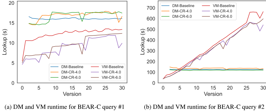
Fig. 14. BEAR-C average query execution time in seconds for VM, DM, and V queries.
