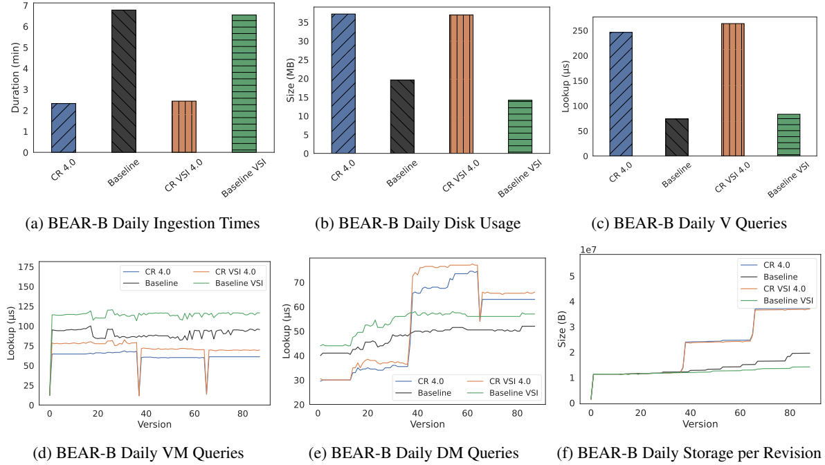
Fig. 11. BEAR-B Daily performance impact on ingestion time, storage, and VM, DM, and V query runtime for the compression using variable size integer (VSI) on both OSTRICH and our multi-snapshot strategy with change ratio \gamma = 4.0 .
