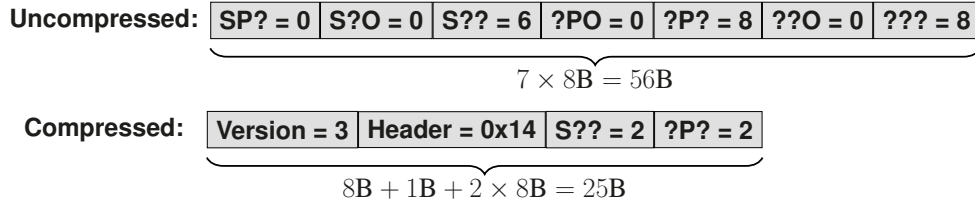
Fig. 5. Representation of the positions vectors for version 3 of our example, without and with compression.
