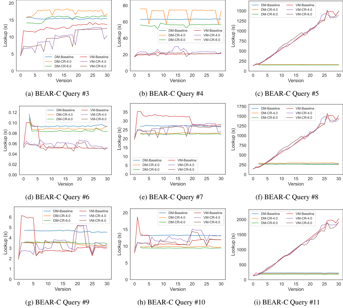
Fig. 15. Individual runtime of DM and VM SPARQL queries for BEAR-C.
