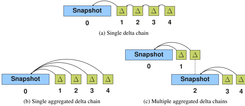
Fig. 4. Delta chain architectures
