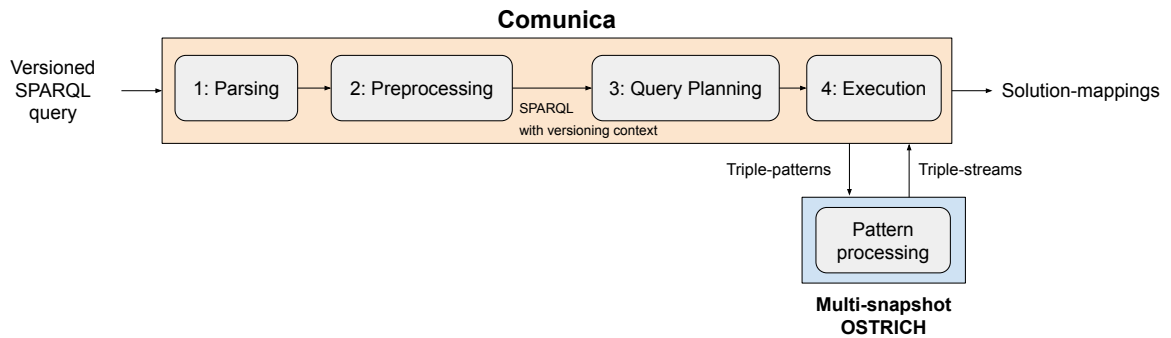
Fig. 6. SPARQL query processing pipeline
