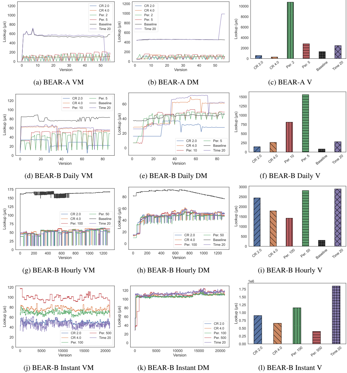
Fig. 9. Query results for the BEAR benchmark
