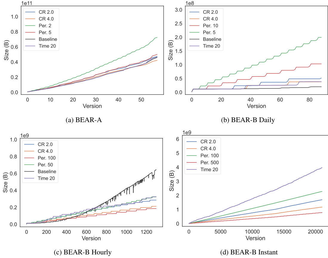
Fig. 8. Disk usage evolution per revision for the BEAR-A and BEAR-B datasets.
