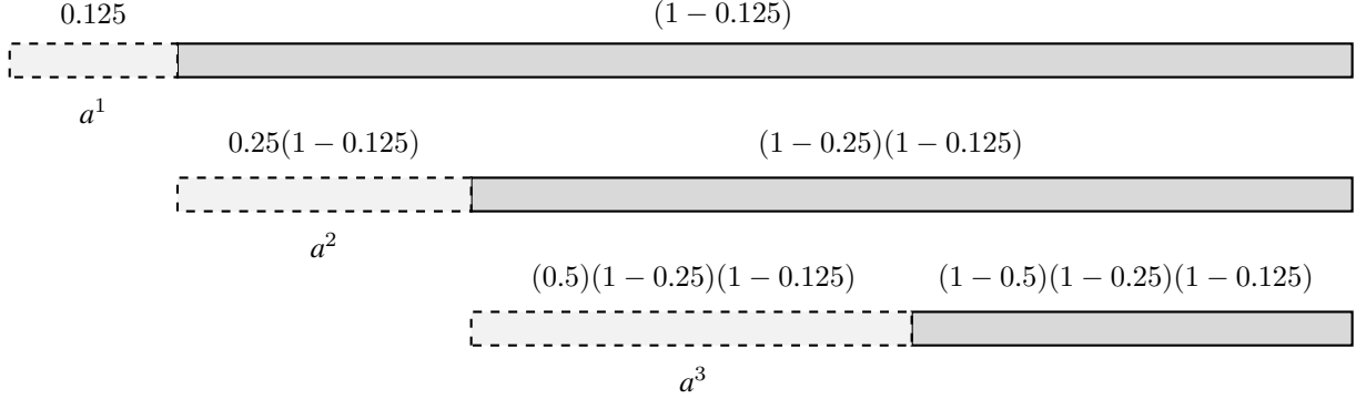
Fig. 4. Toy example of the stick breaking process with values v^1 = 0.125 v^2 = 0.25 v^3 = 0.5 . Starting at the top of the figure, a unit length stick is broken at v^1 . The remainder is then iteratively broken proportionally to draws from the Beta distribution.
