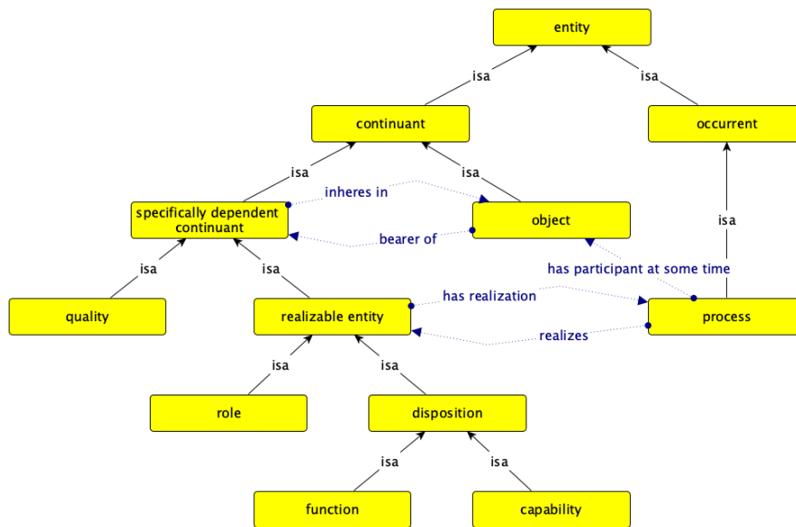
Fig. 1. Fragment of the BFO taxonomy
