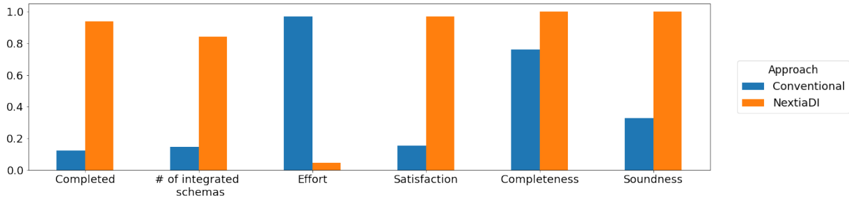
Fig. 23. Aggregated results for the schema integration phase. Completed indicates whether participants finished the task within the available time (higher is better). # of integrated schemas denotes how many schema elements participants managed to integrate in the available time (higher is better). Effort indicates perceived effort to complete the task (lower is better). Satisfaction is used to quantify the perceived satisfaction of running the task with each approach (higher is better). Completeness and Soundness refer to the quality metrics previously introduced.
