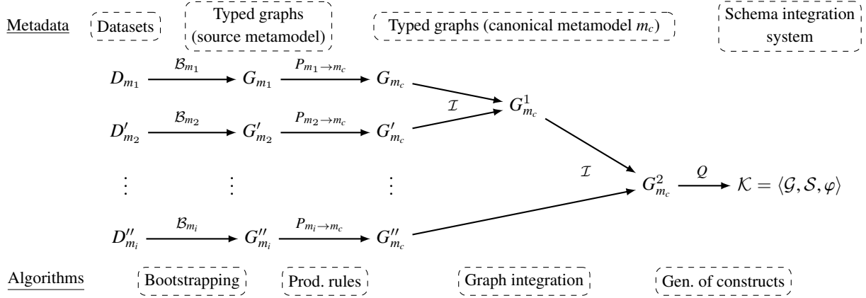
Fig. 3. Formal overview of our approach
