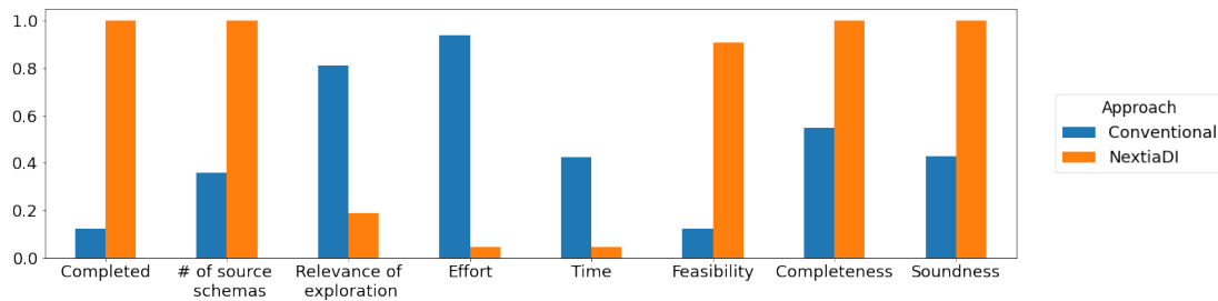
Fig. 22. Aggregated results for the bootstrapping phase. Completed indicates whether participants finished the task within the available time (higher is better). # of source schemas denotes how many schema elements participants managed to bootstrap in the available time (higher is better). Relevance of exploration denotes the need a participant perceived to explore the structure of the sources to conduct the activity (lower is better). Effort and Time indicate, respectively, the perceived effort and time to complete the task (lower is better). Feasibility is used to quantify the perceived feasibility of running the task with the approach at hand (higher is better). Completeness and Soundness refer to the quality metrics previously introduced.
