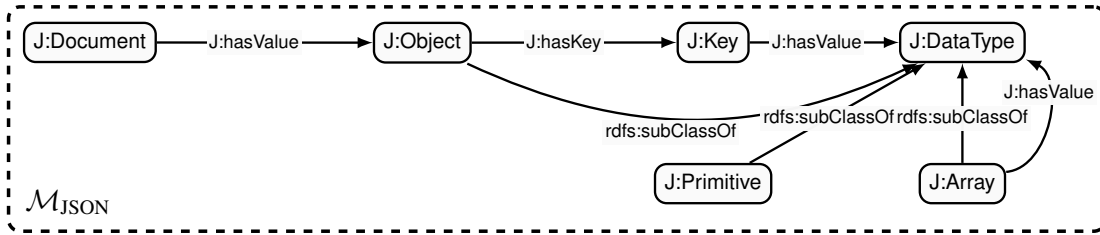
Fig. 5. Metamodel to represent graph-based schemata of JSON datasets (i.e., \mathcal{M}_{\text{JSON}} ) inspired from [55]
