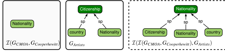
Fig. 17. Result of integrating one integrated data type property from \mathcal{I}(G_{CMOA}, G_{Cooperhewitt}) and G_{Artists}
