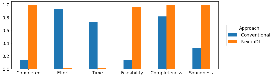
Fig. 24. Aggregated results for the mapping generation phase. Completed indicates whether participants finished the task within the available time (higher is better). Effort and Time indicate, respectively, the perceived effort and time to complete the task (lower is better). Feasible is used to quantify the perceived feasibility of the task in Big Data settings (higher is better). Completeness and Soundness refer to the quality metrics previously introduced.
