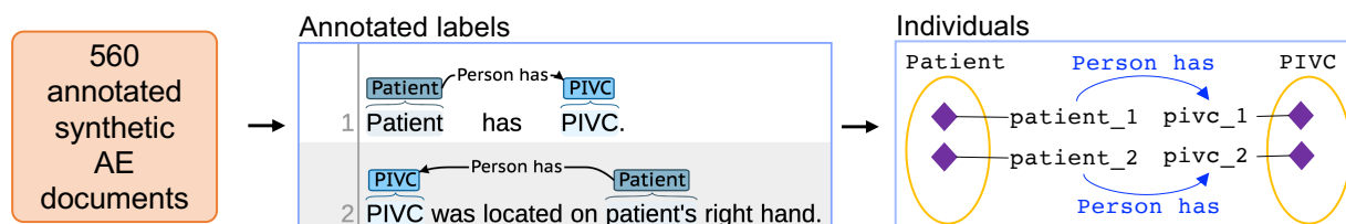
Fig. 2. Using an annotated corpus to populate individuals in a terminology. Each of the 560 documents were translated into an individual and each label within a document was also translated into an individual. In the simplified example, an annotated document has 2 patient labels, 2 PIVC labels, and 2 \xrightarrow{\text{Person has}} relationships linking the labels. Each label is converted into an individual (i.e., a purple diamond) of the corresponding class (i.e., Patient or PIVC yellow circle). Then the labels are linked using the \xrightarrow{\text{Person has}} object property, similarly to how the \xrightarrow{\text{Person has}} relationship links labels in the annotated text.
