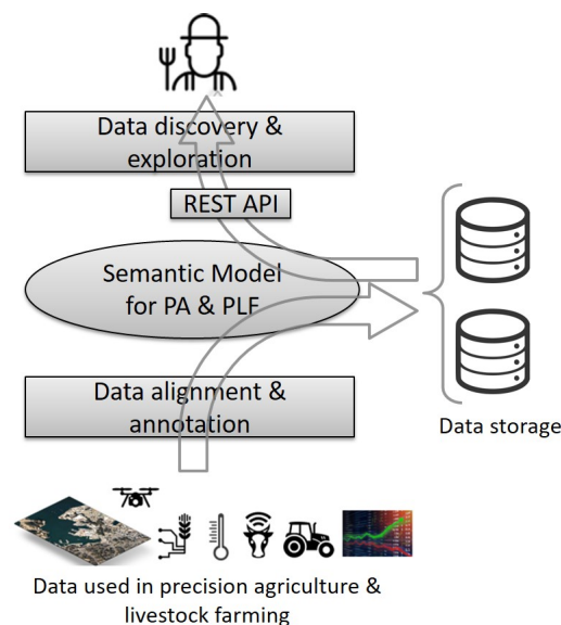
Fig. 3. The role of the Semantic Model for Precision Agriculture and Precision Livestock Farming
