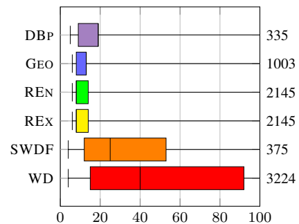
Fig. 7. R-graph sizes (number of nodes) for each set of queries; the value on the right indicates the maximum size
