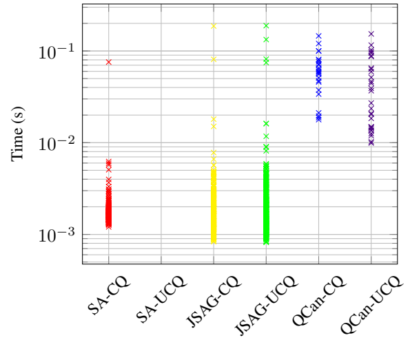
Fig. 9. Runtimes for JSAG, SA and QCan
