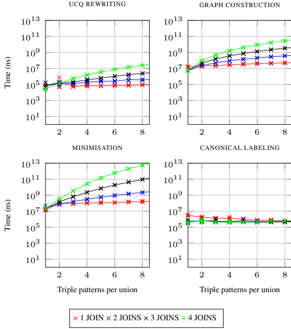
Fig. 10. Times for UCQ stress tests
