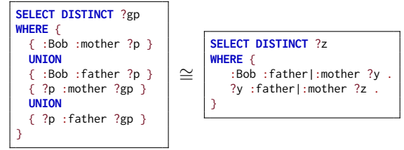
Fig. 2. Example of query congruence
