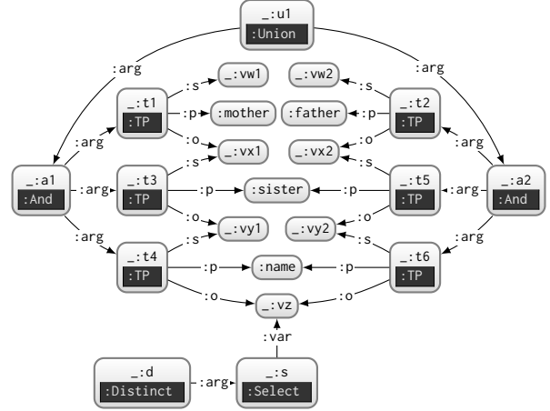
Fig. 3. UCQ (above) and its r-graph (below)
