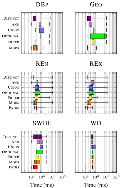
Fig. 8. Runtimes for queries grouped by selected features
