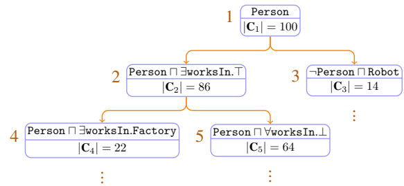
Fig. 3. A fragment of TCT whose nodes are also decorated with the size of the respective cluster of individuals \mathbf{C}_i . Intuitively, the concept descriptions D_i in the various nodes could be roughly mapped ( CN_i \equiv D_i ) to the following names, respectively: CN_2 : \text{Employee} , CN_3 : \text{Robot} , CN_4 : \text{Worker} , CN_5 : \text{Freelance} .
