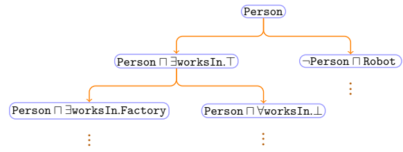
Fig. 2. A fragment of a TCT.
