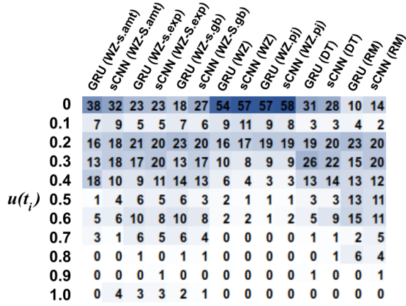
Fig. 6. (Best viewed in colour) Distribution of additional true positives (compared against Gamback et al.) identified by CNN+sCNN (sCNN for shorthand) and CNN+GRU (GRU) over different ranges of uniqueness scores (Equation 1) when using the Word2Vec embeddings. Each row in the heatmap corresponds to a uniqueness score range. Each column corresponds to a method-dataset pair. The numbers in each column sum up to 100% while the colour scale within each cell is determined by the number in that cell.
