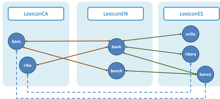
Fig. 4. Example of translation candidates between ES and CA (EN as pivot language) in Apertium RDF. We do not represent here the translation sets for simplicity. The dashed connectors show the direct ES-CA translations.
