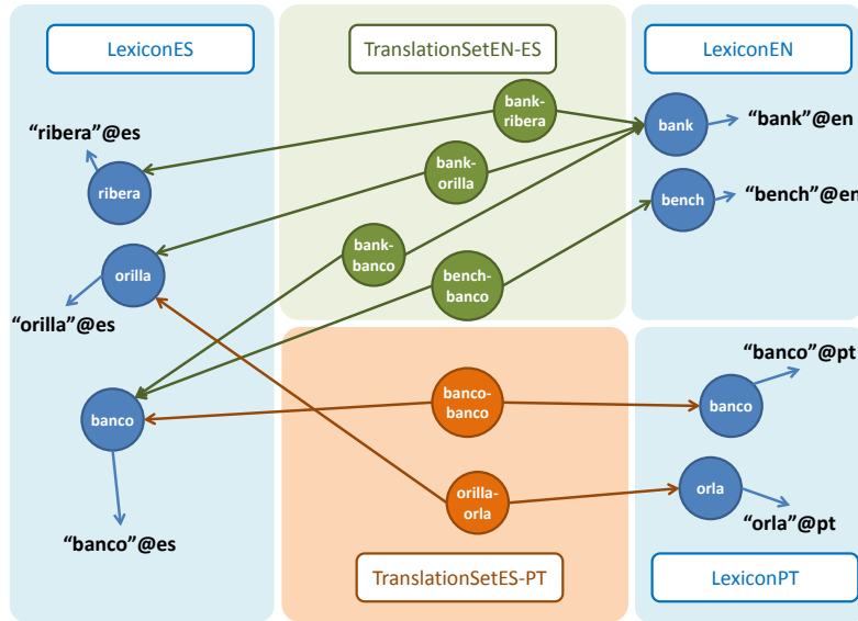
Fig. 3. Simplified representation of the path between some lexical entries in EN and PT (disconnected in the original Apertium dictionaries).
