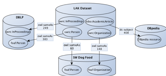
Fig. 2 : Links in the LAK Dataset 27
