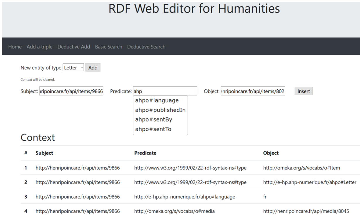
Fig. 8. A screenshot of RDFWebEditor4Humanities.
